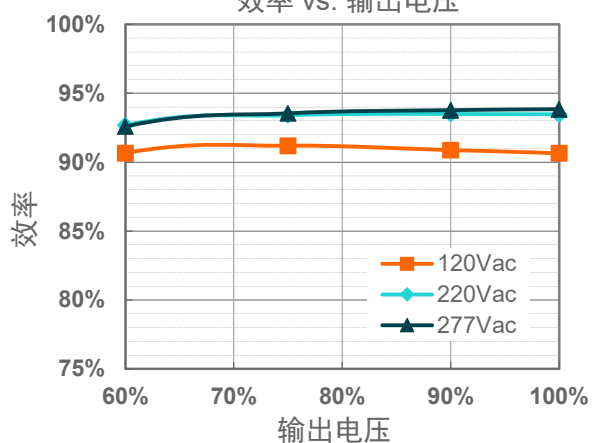
EUM-240S150Bx( I_o=1050mA )
