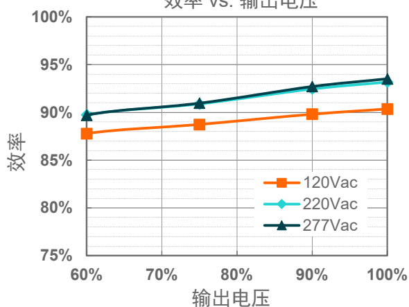
EUM-240S150Bx( I_o=1500mA )
