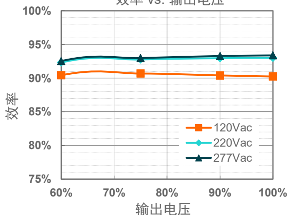
EUM-240S670Bx( I_o=4200mA )
