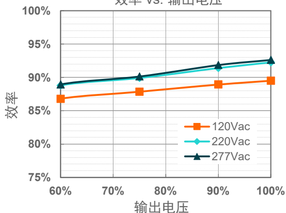
EUM-240S670Bx( I_o=6700mA )
